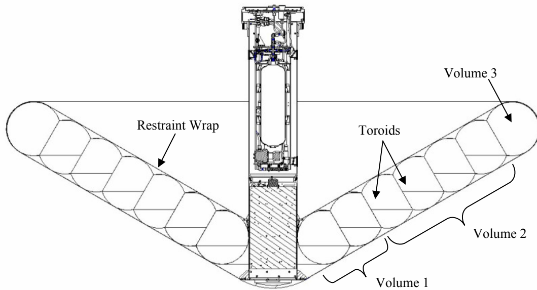
Figure 4. IRVE cross-section.
